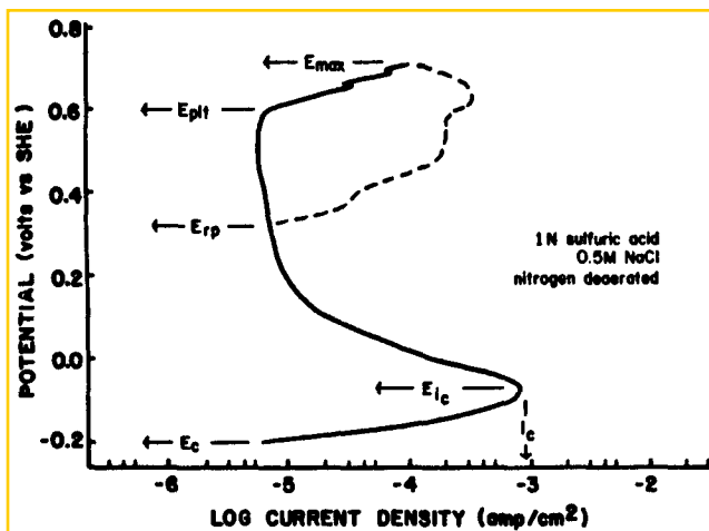
FIGURE 1. Schematic diagram of the CPPT. The characteristic parameters that define the curve are: E_c = open circuit potential; i_c = critical passivation CD; E_p = potential corresponding to i_c ; E_{pit} = pitting potential; E_{max} = potential at which scan direction is reversed ( i = 10^{-4} A/cm 2 ); and E_{rep} = repassivation potential.
