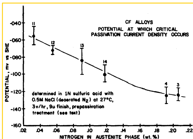
FIGURE 8. Potential at which i_a occurs for solution-treated CF alloys as a function of austenite nitrogen content. Number above each scatter bar identifies the specific CF alloy.
